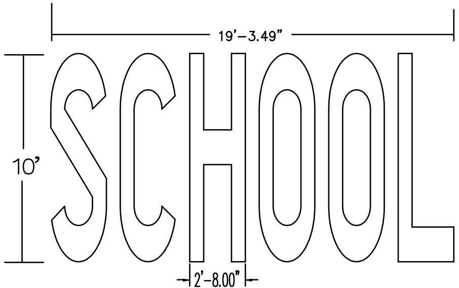
10' SCHOOL Legend 90 mil HotTape Item # HT894904 125 mil HotTape Item # HT894168
