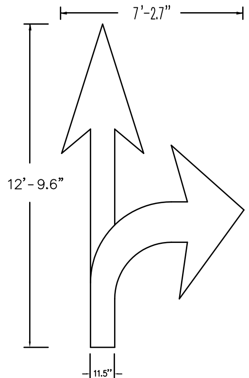
12.75' Combination Arrow Right 90 mil HotTape Item # HT894752 125 mil HotTape Item # HT894068
