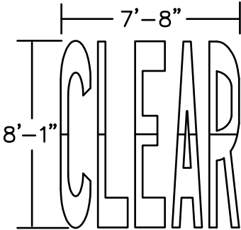
8' CLEAR Legend 90 mil HotTape Item # HT894806 125 mil HotTape Item # HT894112
