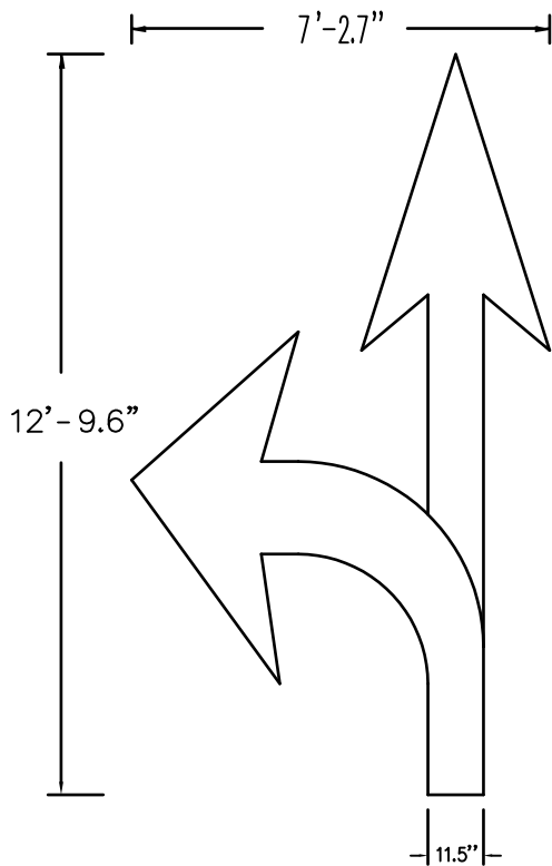
12.75' Combination Arrow Left 90 mil HotTape Item # HT894748 125 mil HotTape Item # HT894064
