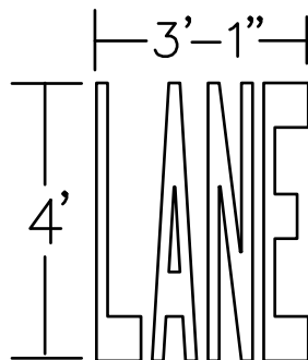
4' LANE Legend 90 mil HotTape Item # HT895118
