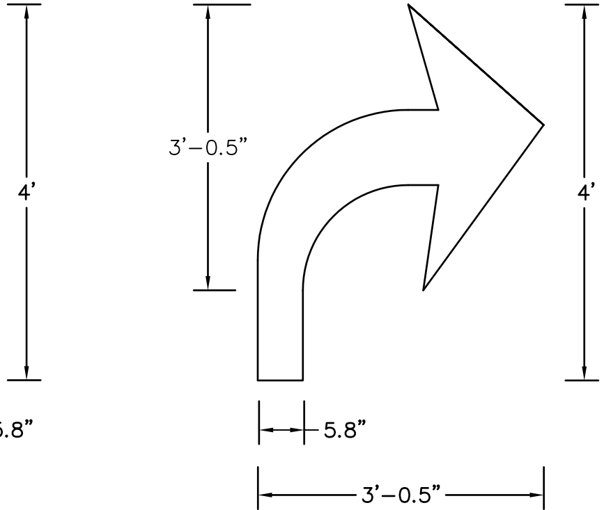
4' Reversible Curved Arrow (non-beaded) 90 mil HotTape Item # HT895120 125 mil HotTape Item # HT894170
