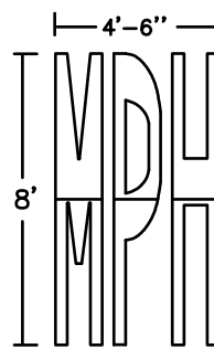
8' MPH Legend 90 mil HotTape Item # HT894838 125 mil HotTape Item # HT894128
