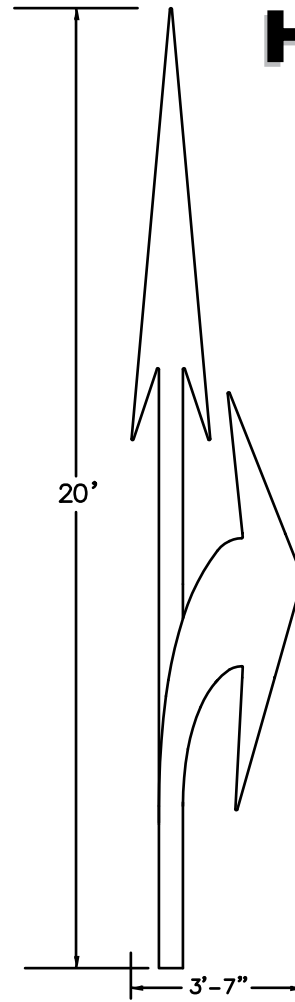
20' Reversible Elongated Combi Arrow (non-beaded) 90 mil HotTape Item # HT894776 125 mil HotTape Item # HT894088
