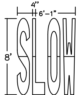
8' SLOW Legend 90 mil HotTape Item # HT894864 125 mil HotTape Item # HT894144
