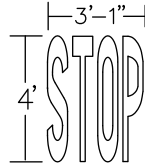
4' STOP Legend 90 mil HotTape Item # HT895276 125 mil HotTape Item # HT895512
