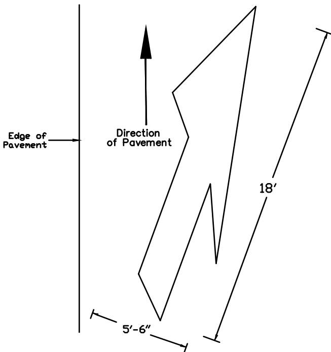
18' Left Lane Drop Arrow 90 mil HotTape Item # HT894762 125 mil HotTape Item # HT894078
