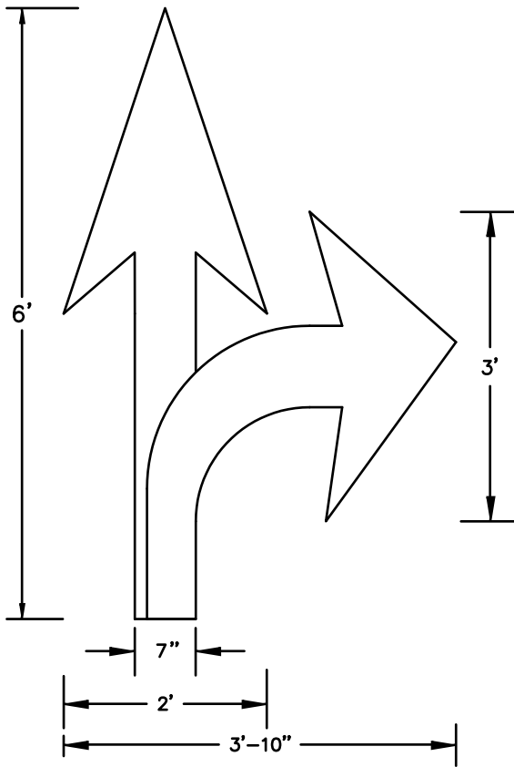
6' Reversible Combination Arrow 90 mil HotTape Item # HT895280 125 mil HotTape Item # HT894176
