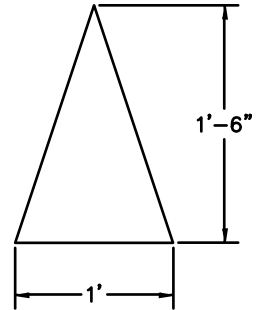
12" x 18" Shark Teeth 90 mil HotTape Item # HT896288 125 mil HotTape Item # HT896289
