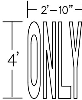
4' ONLY Legend 90 mil HotTape Item # HT895117 125 mil HotTape Item # HT895511
