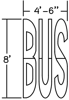
8' BUS Legend 90 mil HotTape Item # HT894802 125 mil HotTape Item # HT894110
