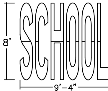
8' SCHOOL Legend 90 mil HotTape Item # HT894900 125 mil HotTape Item # HT894166
