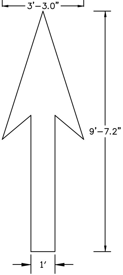
9.6' Straight Arrow 90 mil HotTape Item # HT894898 125 mil HotTape Item # HT894164
