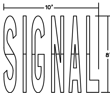
8' SIGNAL Legend 90 mil HotTape Item # HT894860 125 mil HotTape Item # HT894142
