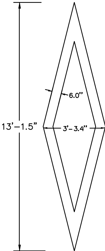
13' HOV Designated Lane 90 mil HotTape Item # HT894756 125 mil HotTape Item # HT894074
