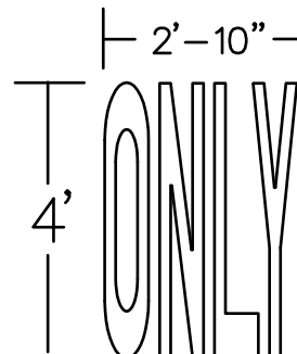
4' ONLY Legend 90 mil HotTape Item # HT895117
