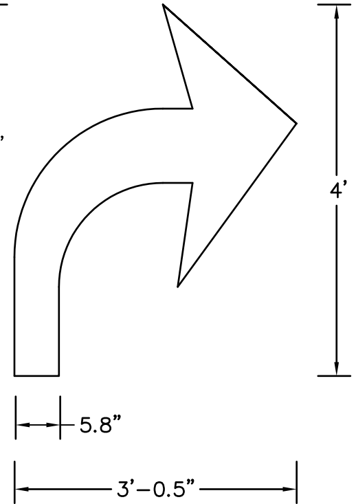
4' Curved Arrow Right 90 mil HotTape Item # HT895124 125 mil HotTape Item # HT894174
