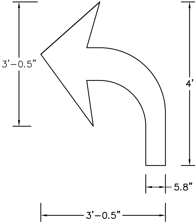
4' Curved Arrow Left 90 mil HotTape Item # HT895122 125 mil HotTape Item # HT894172
