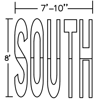
8' SOUTH Legend 90 mil HotTape Item # HT894867 125 mil HotTape Item # HT894143
