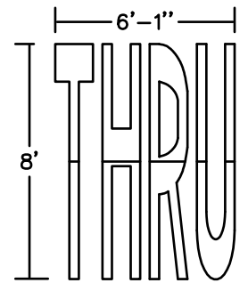
8' THRU Legend 90 mil HotTape Item # HT894872 125 mil HotTape Item # HT894148
