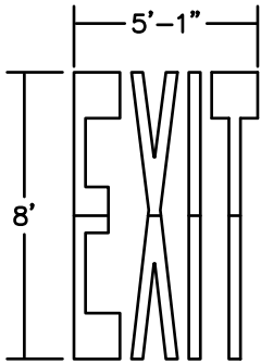
8' EXIT Legend 90 mil HotTape Item # HT894810 125 mil HotTape Item # HT894114
